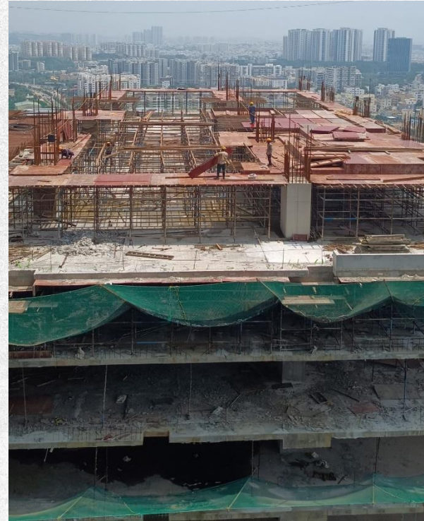
Tower C level 20th floor shuttering works in progress
