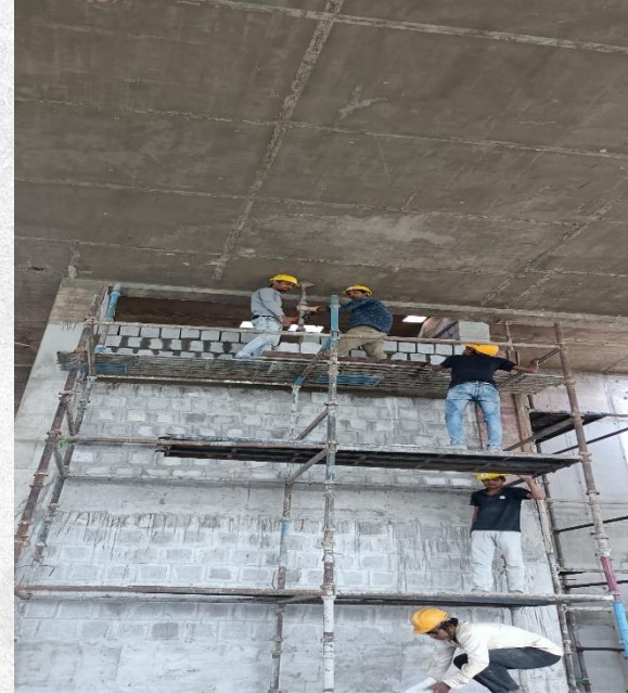
Tower -A L-37 pressurization shaft brick works in progress.
